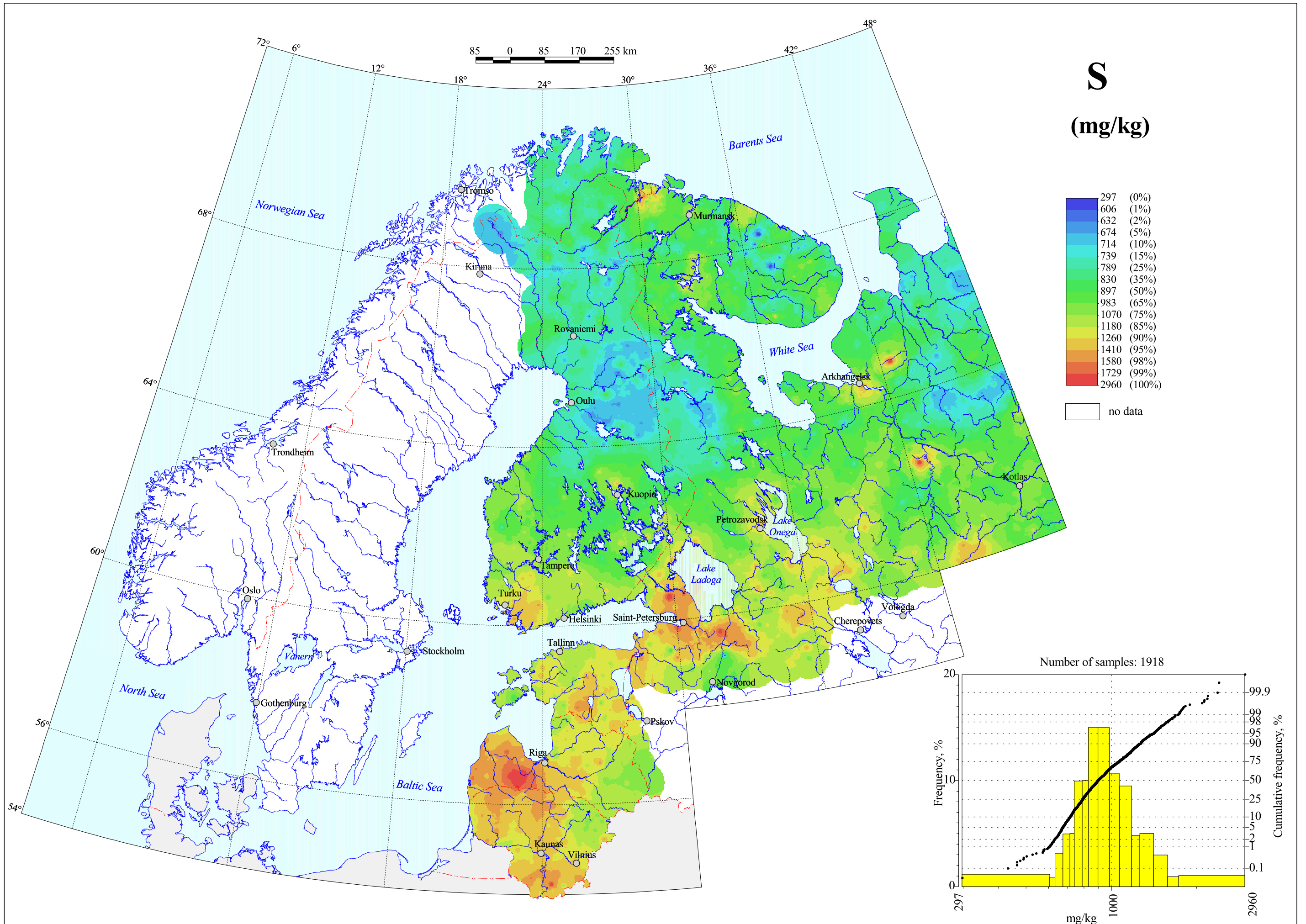
Sulphur in Terrestrial Moss, Total Content
